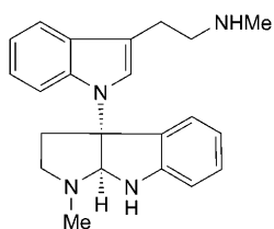
Psychotriasine
